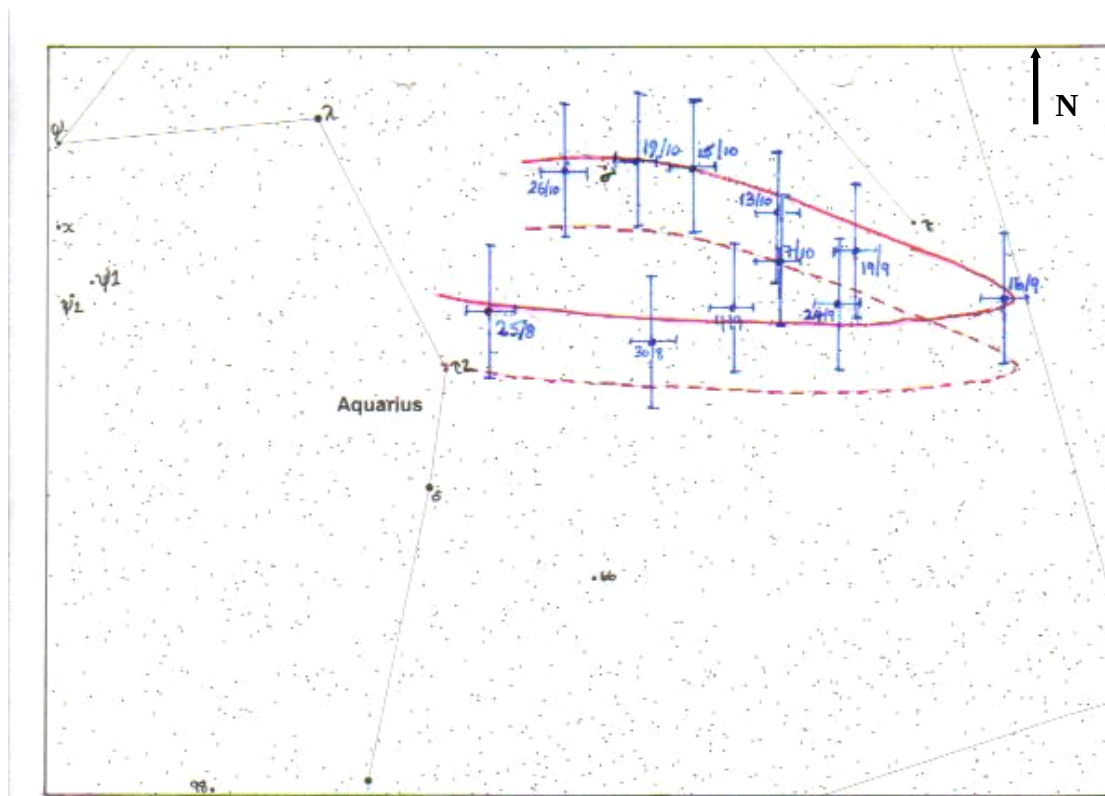
Figure 2 : Apparent motion of Mars, 25/8/03 to 26/10/03
